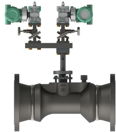
Dual Transmitter
